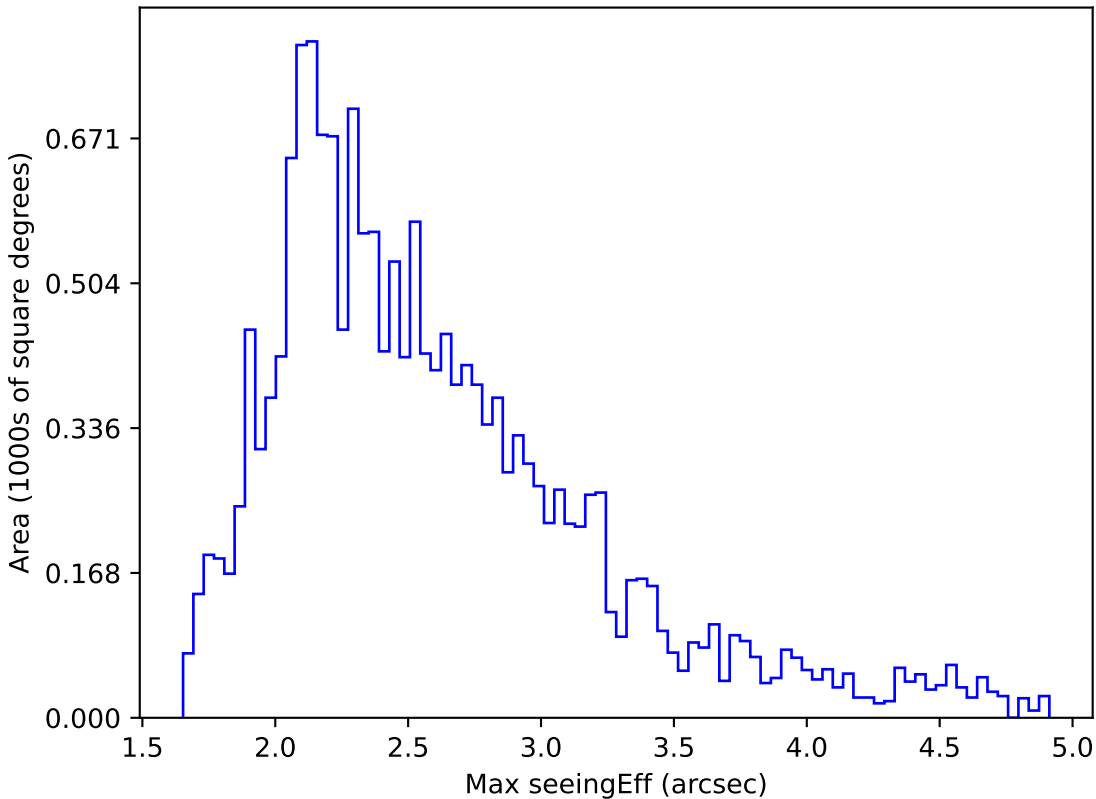
noroll_mjdp365_v3.4_10yrs WFD i band: Max seeingEff
