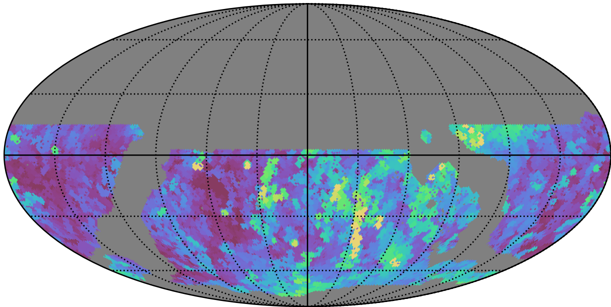
noroll_mjdp365_v3.4_10yrs WFD g band: Max seeingEff
