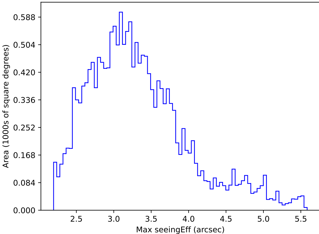
noroll_mjdp365_v3.4_10yrs WFD all bands: Max seeingEff
