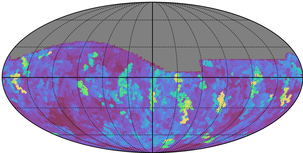
noroll_mjdp365_v3.4_10yrs All sky z band: Max seeingEff
