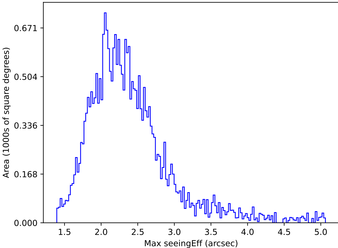
noroll_mjdp365_v3.4_10yrs All sky z band: Max seeingEff
