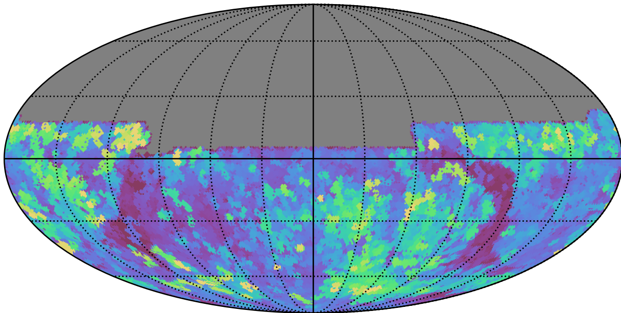
noroll_mjdp365_v3.4_10yrs All sky u band: Max seeingEff
