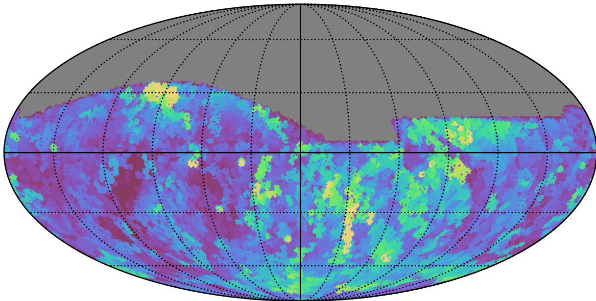
noroll_mjdp365_v3.4_10yrs All sky g band: Max seeingEff
