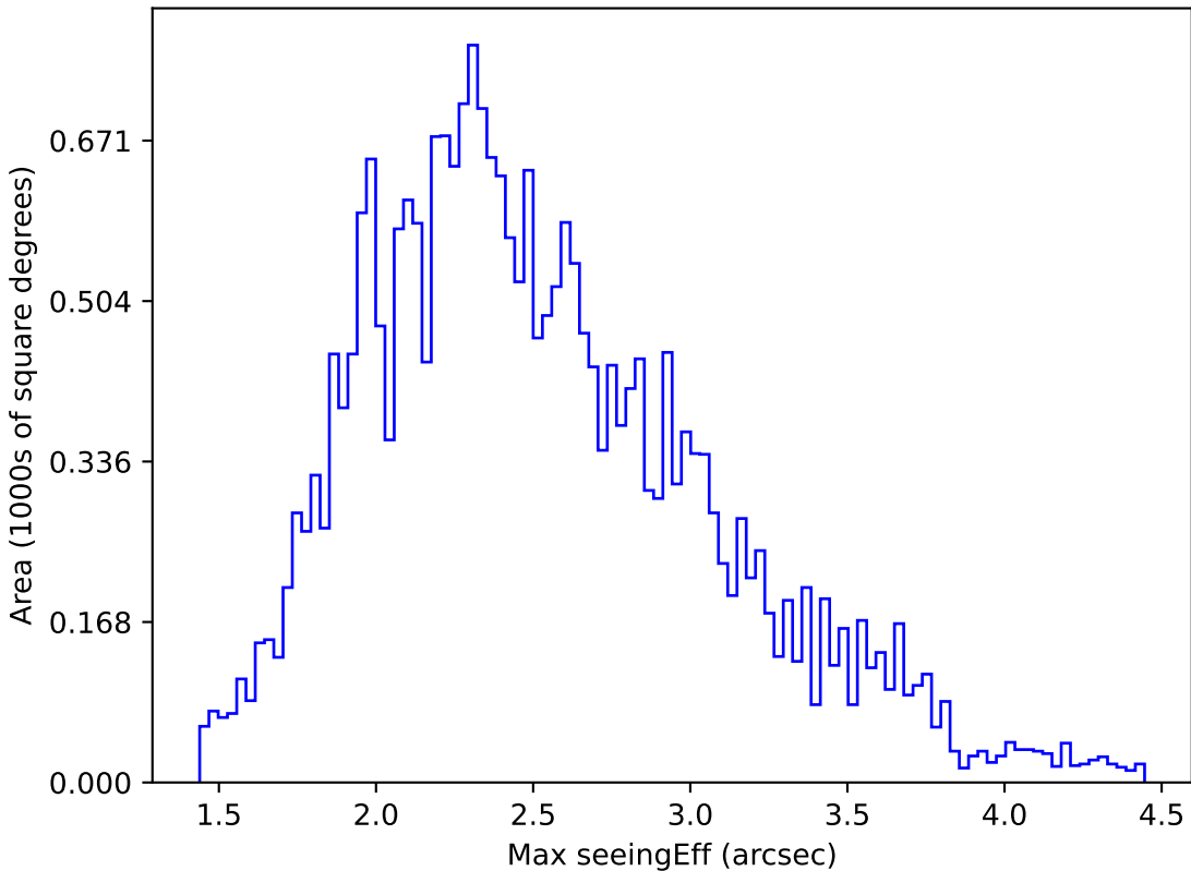
noroll_mjdp365_v3.4_10yrs All sky g band: Max seeingEff
