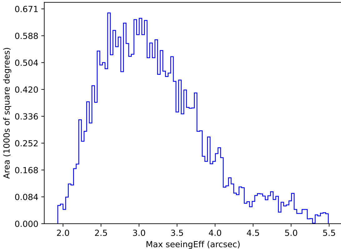
noroll_mjdp365_v3.4_10yrs All sky all bands: Max seeingEff
