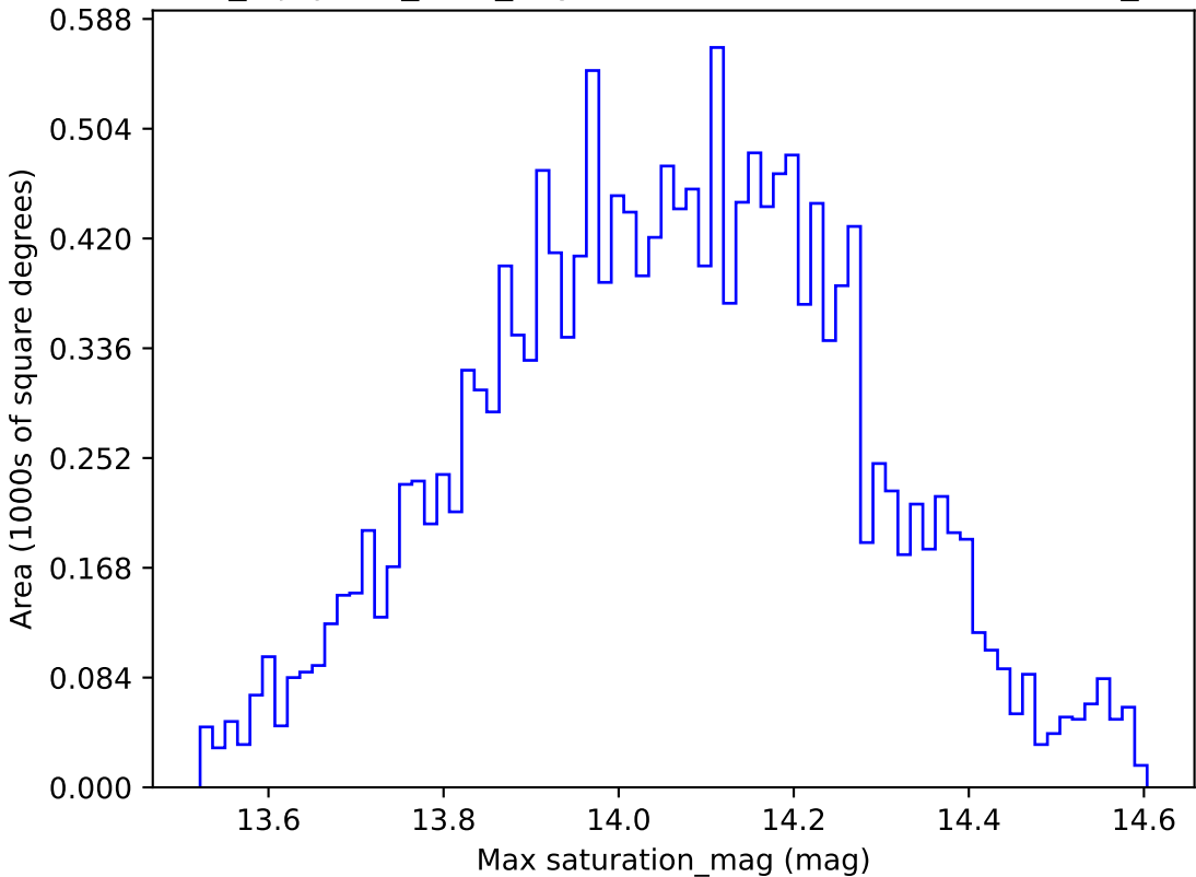
noroll_mjdp365_v3.4_10yrs WFD u band: Max saturation_mag
