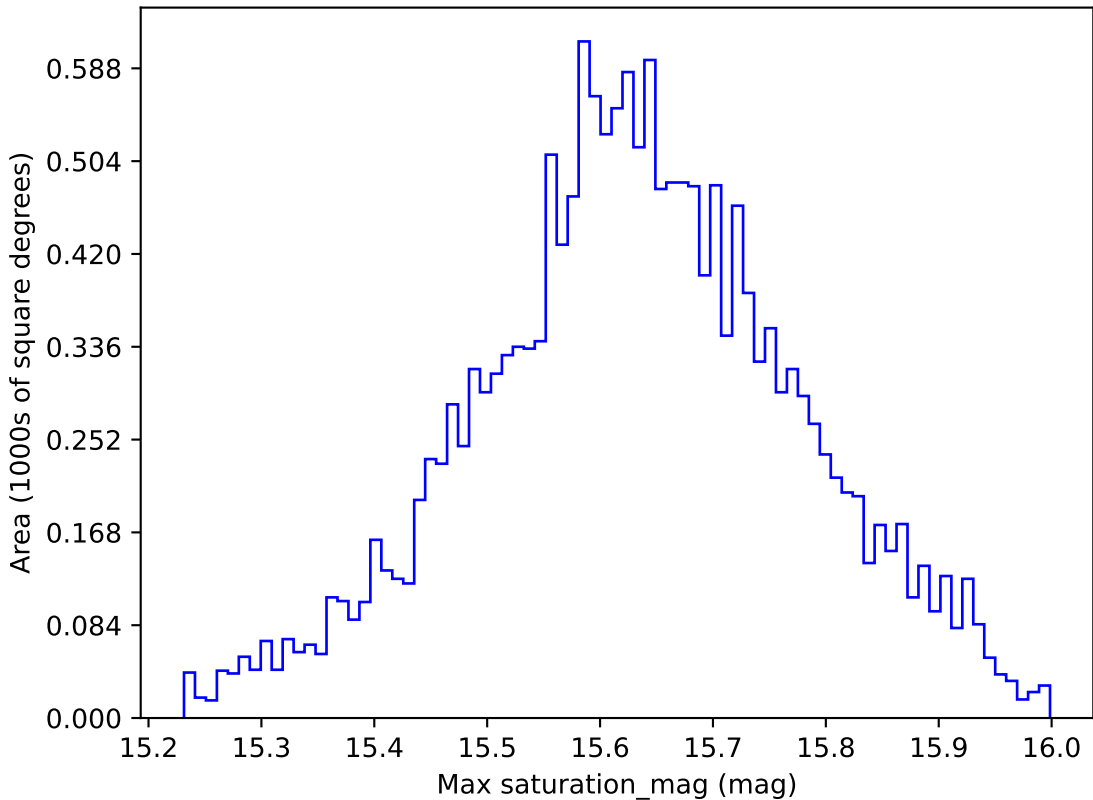
noroll_mjdp365_v3.4_10yrs WFD i band: Max saturation_mag
