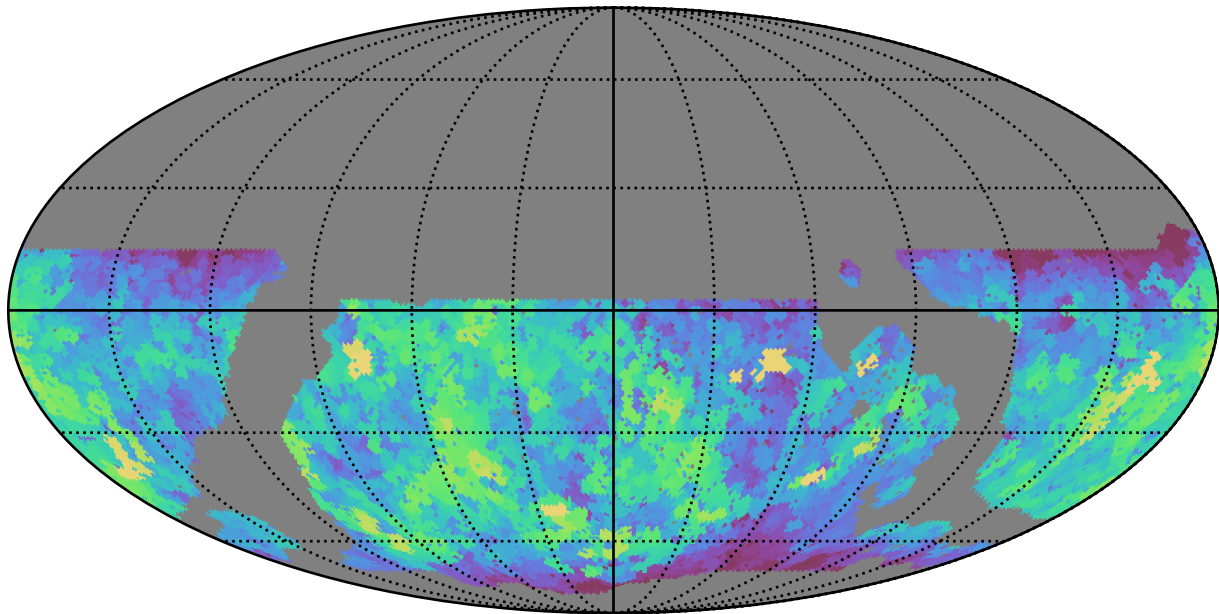
noroll_mjdp365_v3.4_10yrs WFD g band: Max saturation_mag
