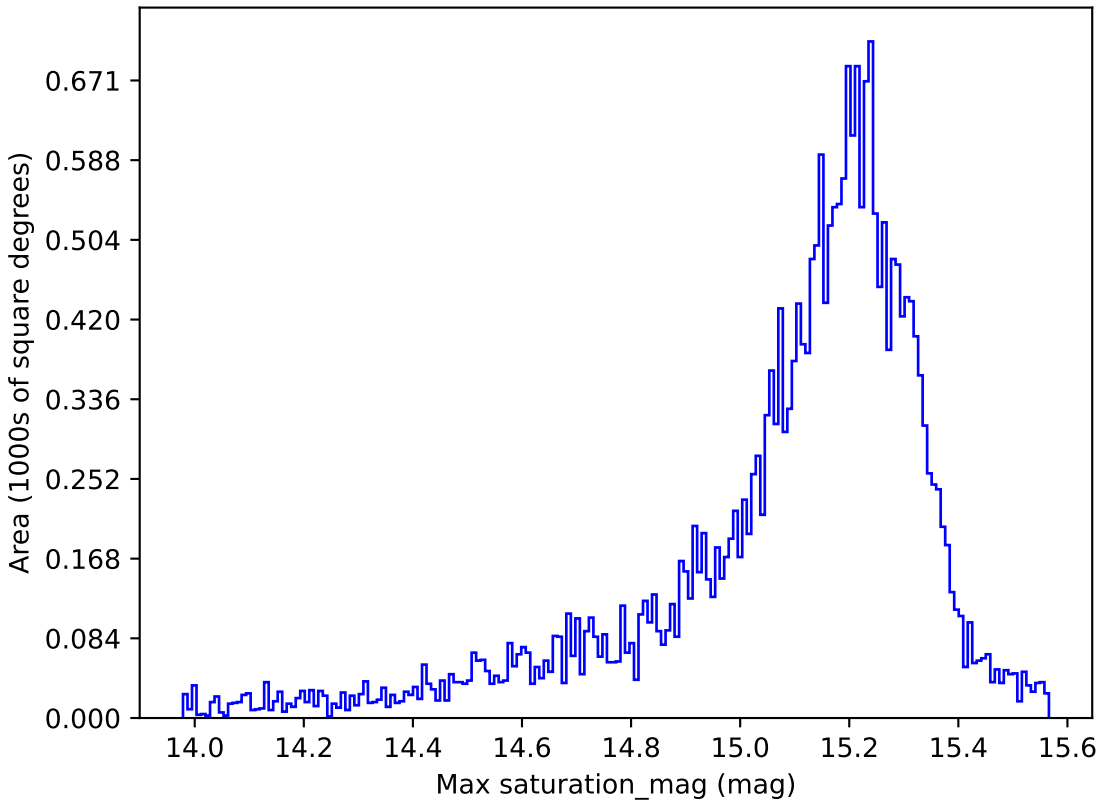
noroll_mjdp365_v3.4_10yrs All sky z band: Max saturation_mag
