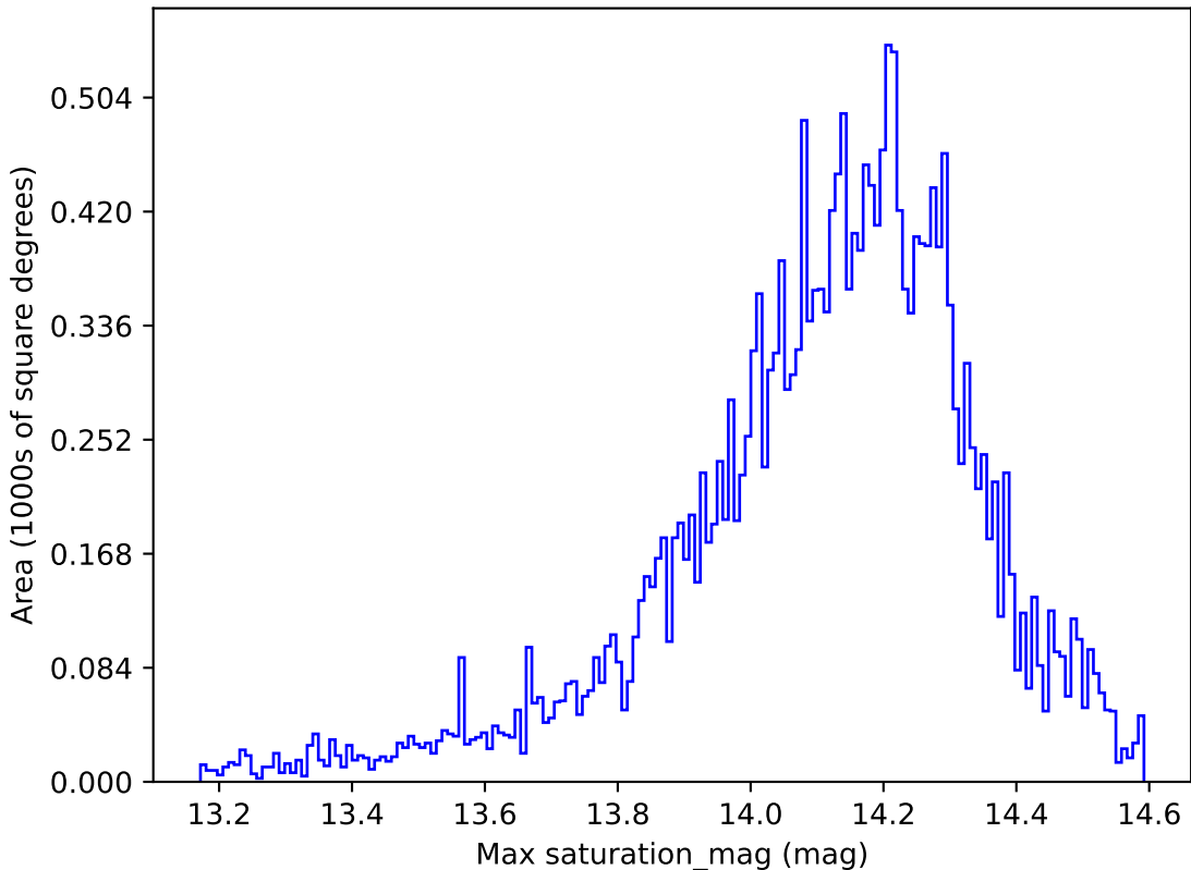
noroll_mjdp365_v3.4_10yrs All sky y band: Max saturation_mag
