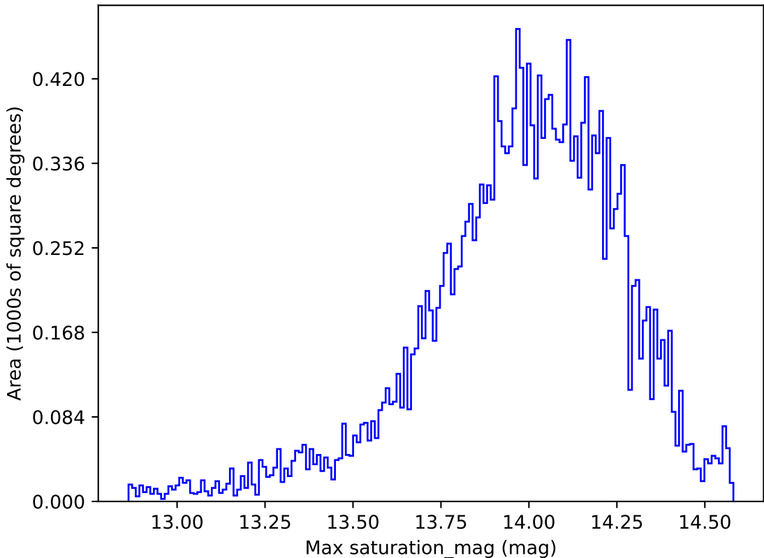
noroll_mjdp365_v3.4_10yrs All sky u band: Max saturation_mag
