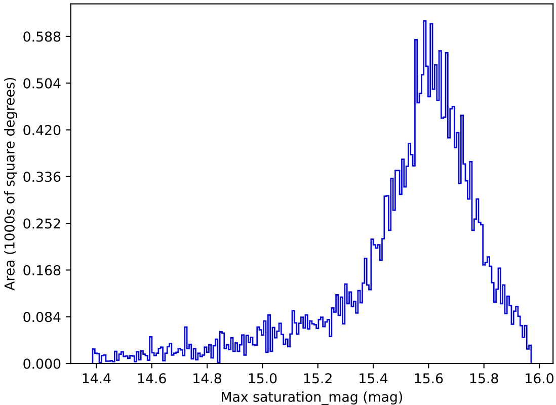
noroll_mjdp365_v3.4_10yrs All sky i band: Max saturation_mag
