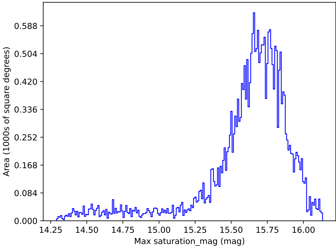
noroll_mjdp365_v3.4_10yrs All sky g band: Max saturation_mag
