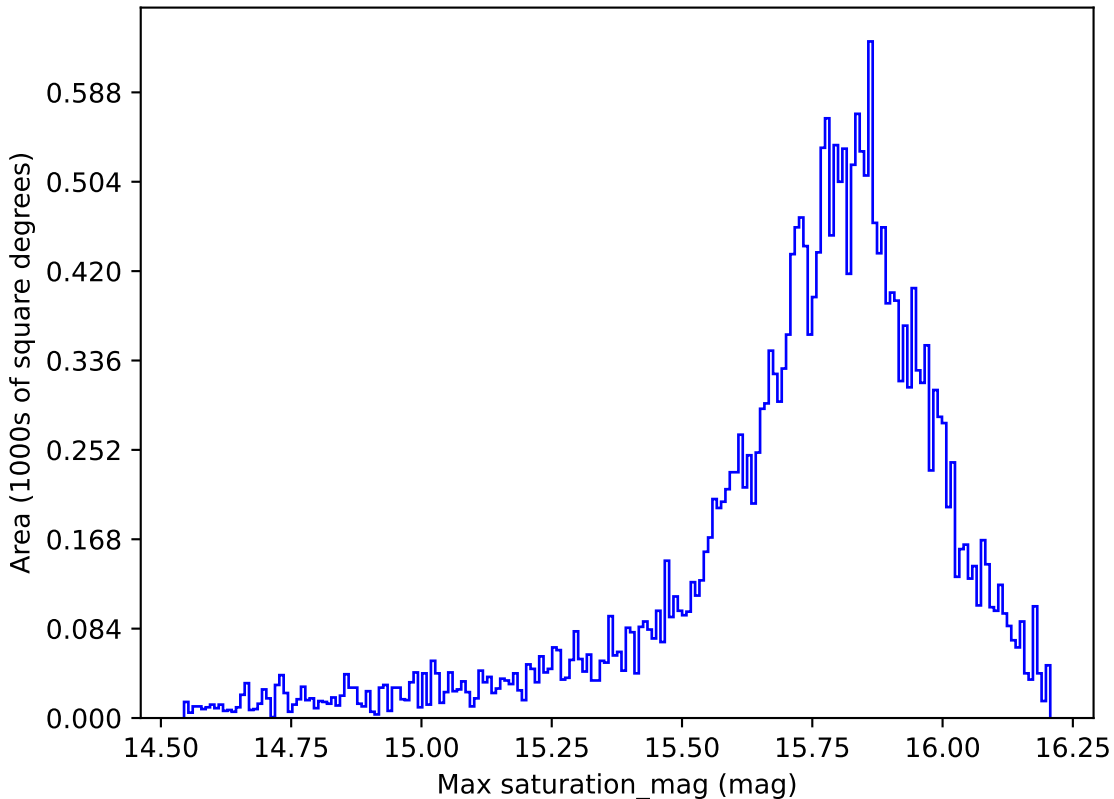
noroll_mjdp365_v3.4_10yrs All sky all bands: Max saturation_mag
