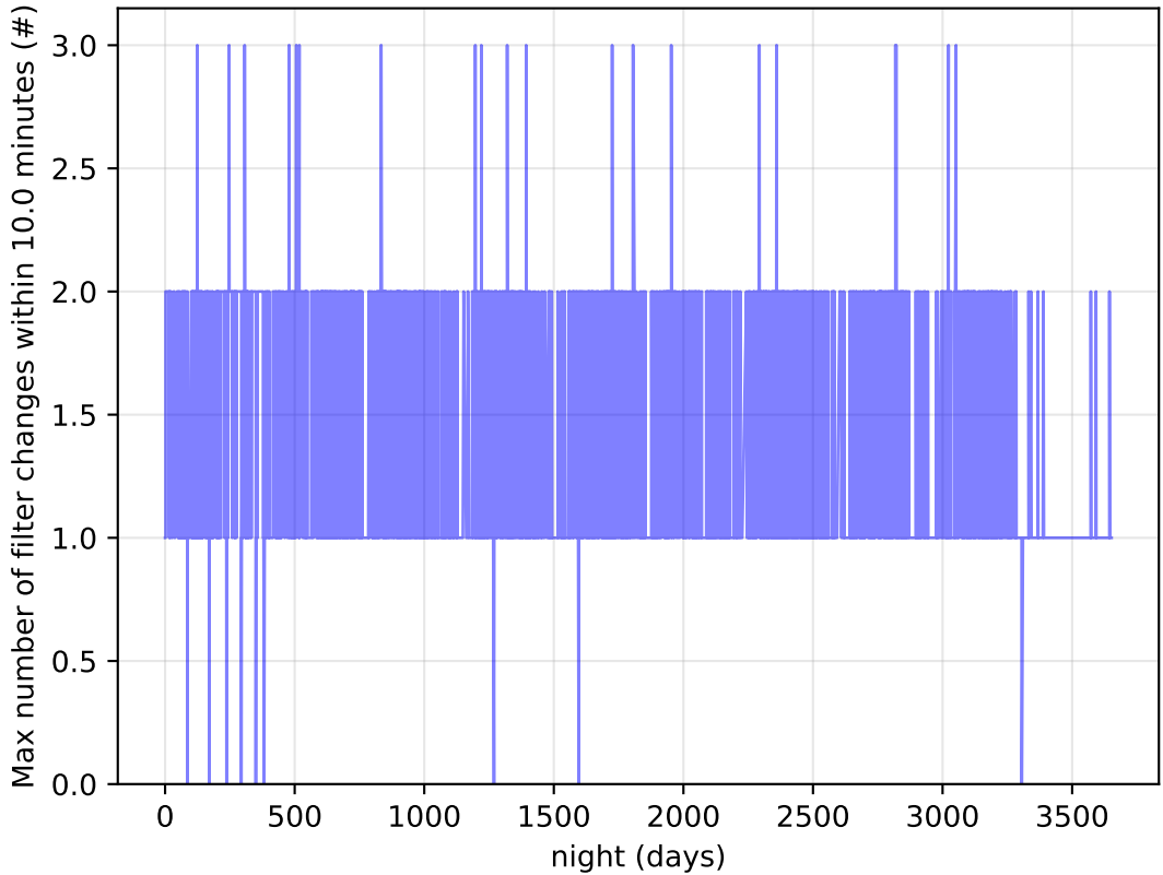
noroll_mjdp365_v3.4_10yrs Per Night: Max number of filter changes within 10.0 minutes
