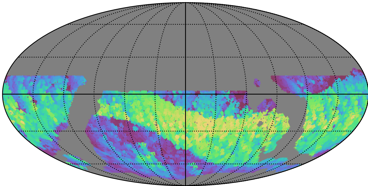
noroll_mjdp365_v3.4_10yrs WFD z band: Max normairmass
