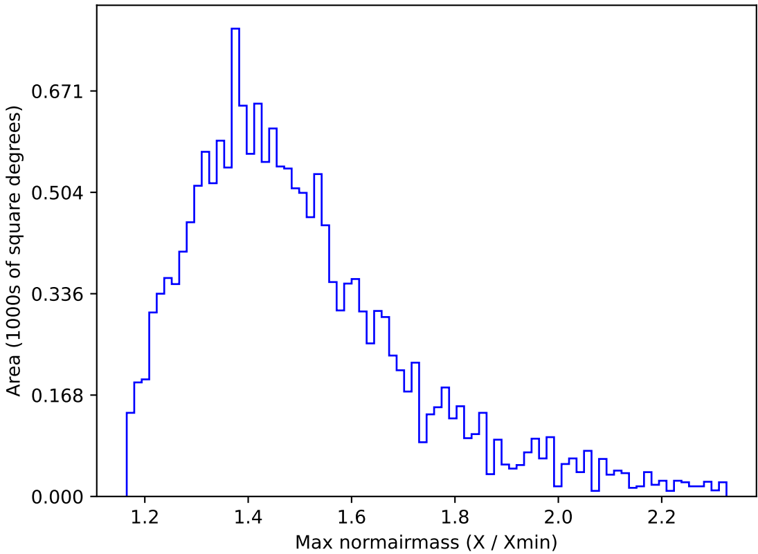
noroll_mjdp365_v3.4_10yrs WFD u band: Max normairmass
