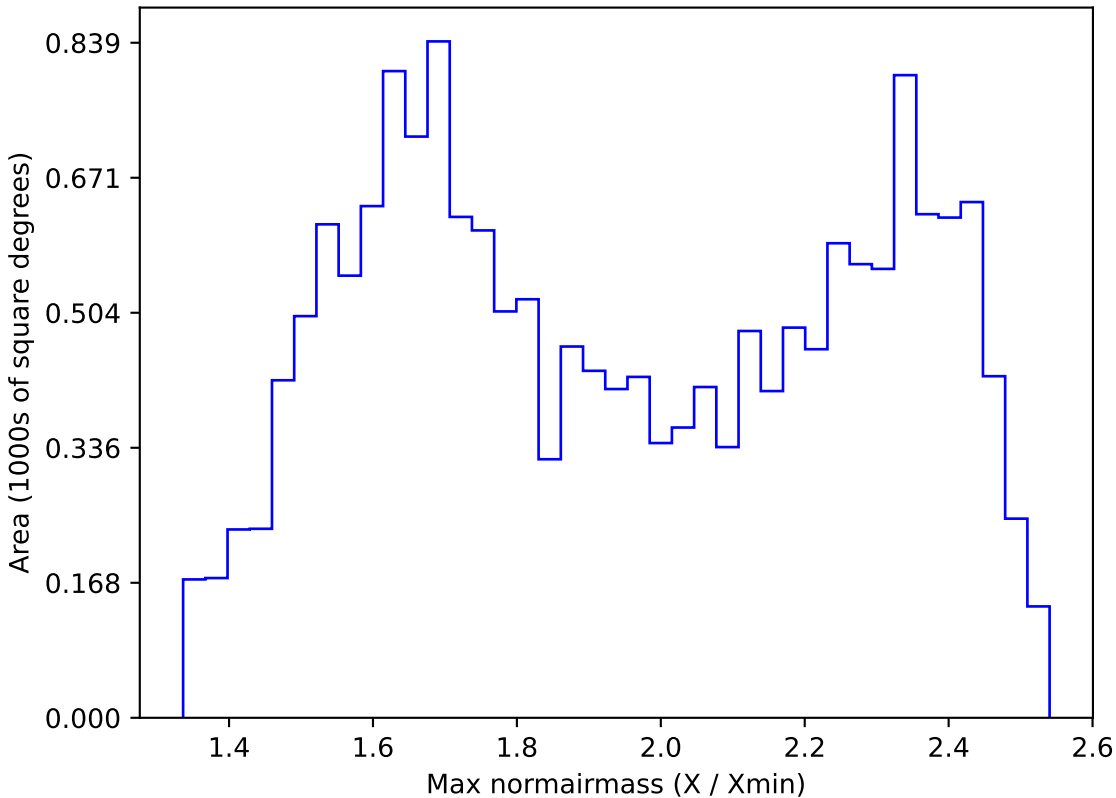
noroll_mjdp365_v3.4_10yrs WFD r band: Max normairmass
