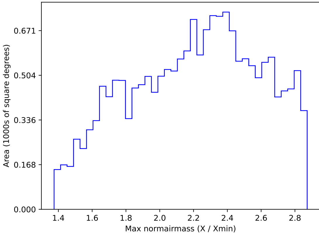
noroll_mjdp365_v3.4_10yrs WFD i band: Max normairmass
