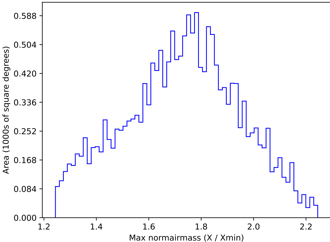
noroll_mjdp365_v3.4_10yrs WFD g band: Max normairmass
