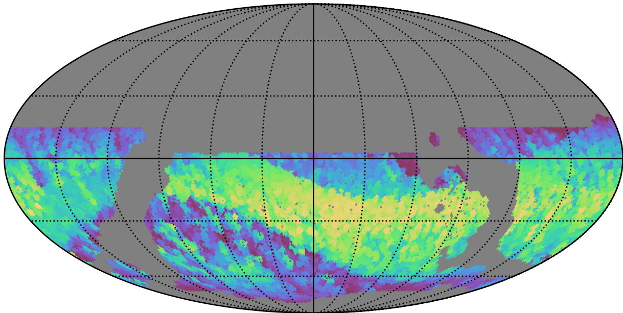
noroll_mjdp365_v3.4_10yrs WFD all bands: Max normairmass
