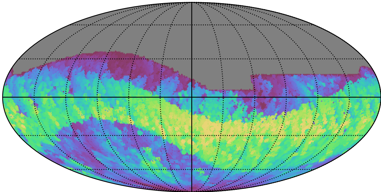
noroll_mjdp365_v3.4_10yrs All sky z band: Max normairmass
