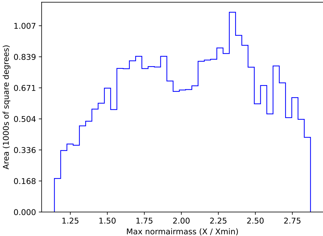
noroll_mjdp365_v3.4_10yrs All sky z band: Max normairmass
