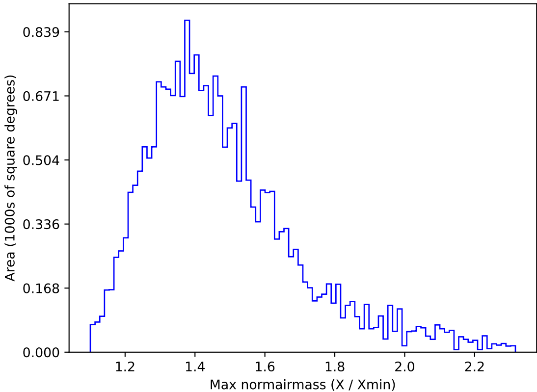
noroll_mjdp365_v3.4_10yrs All sky u band: Max normairmass
