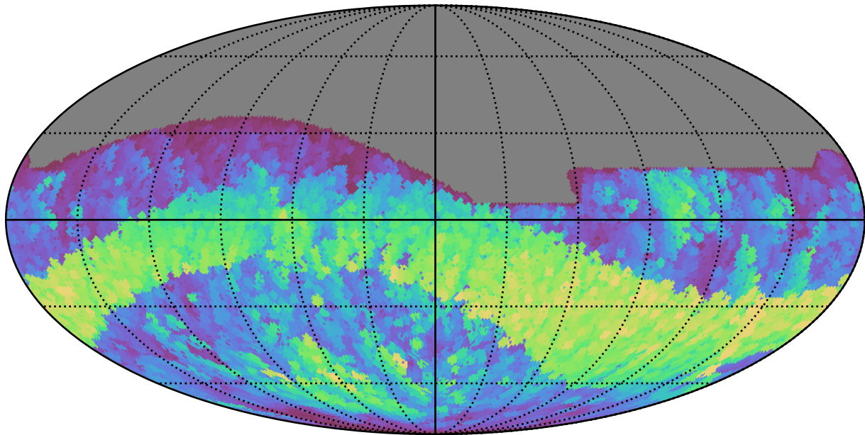
noroll_mjdp365_v3.4_10yrs All sky r band: Max normairmass
