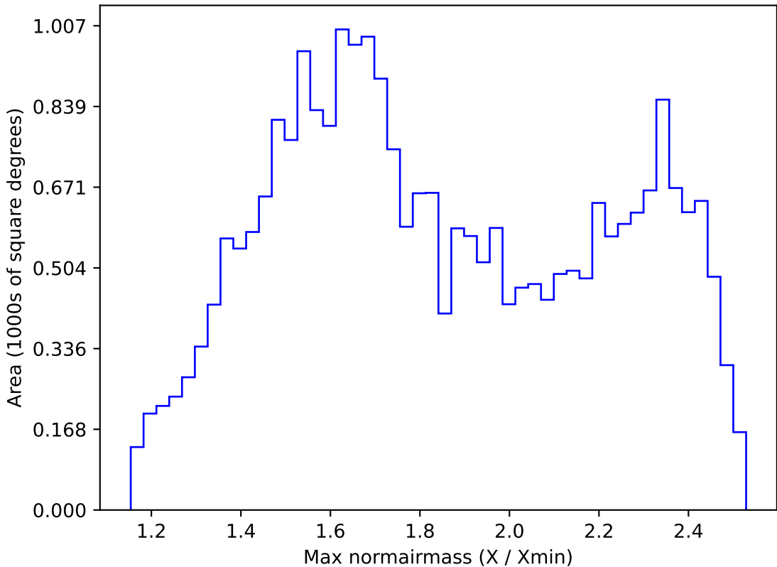
noroll_mjdp365_v3.4_10yrs All sky r band: Max normairmass
