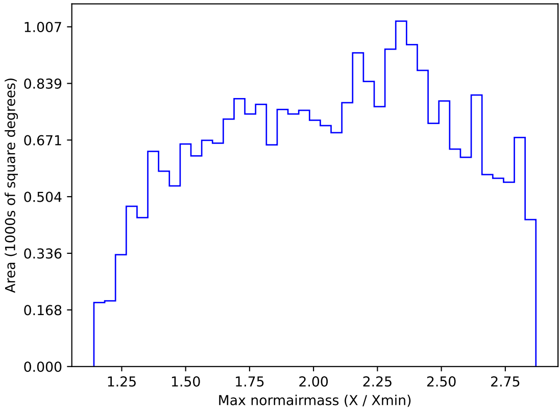
noroll_mjdp365_v3.4_10yrs All sky i band: Max normairmass
