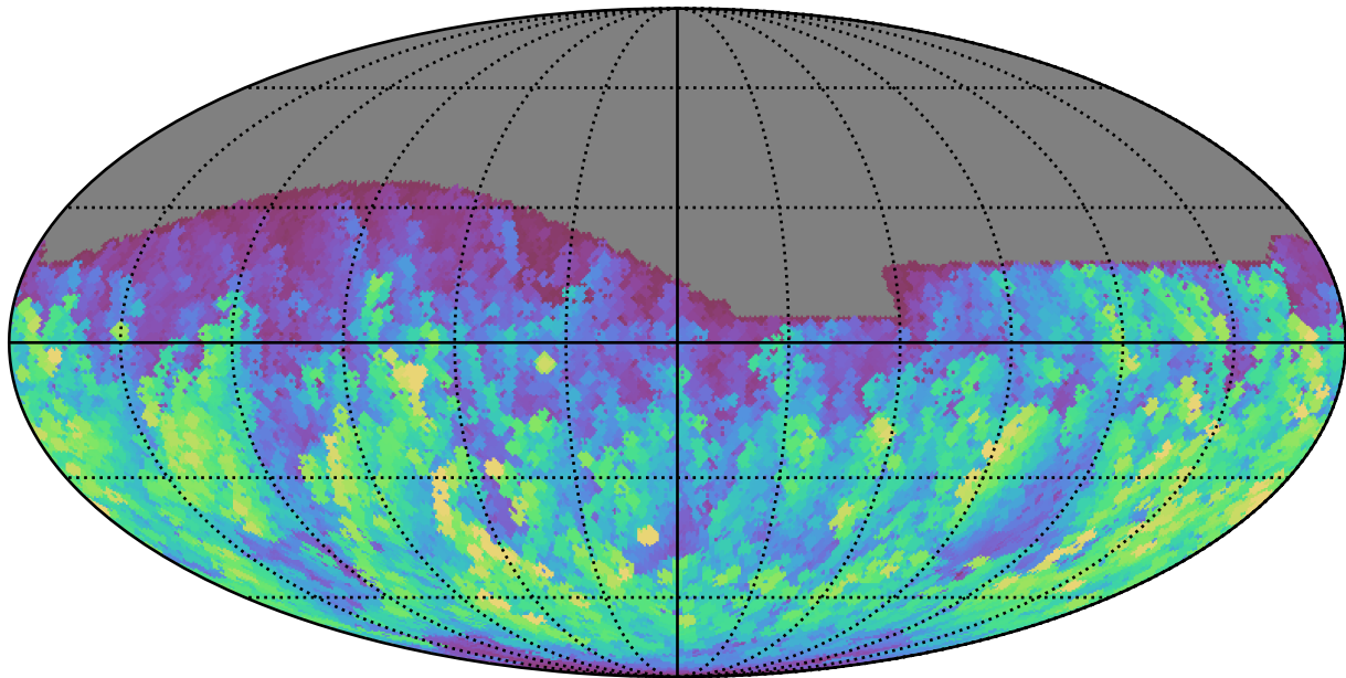
noroll_mjdp365_v3.4_10yrs All sky g band: Max normairmass
