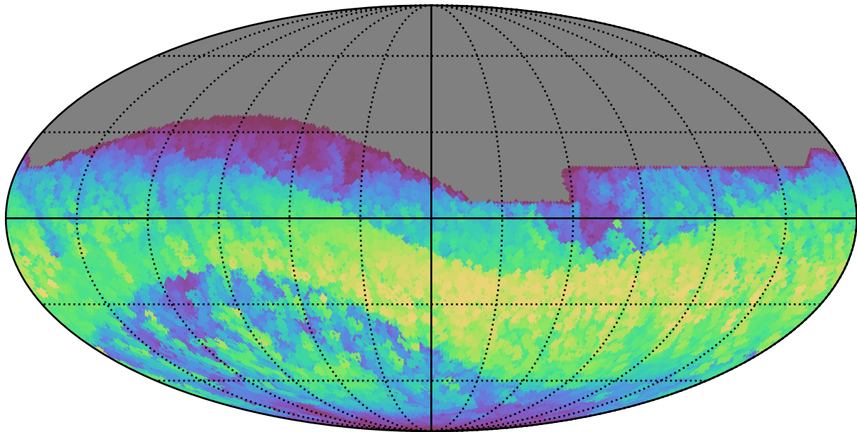
noroll_mjdp365_v3.4_10yrs All sky all bands: Max normairmass
