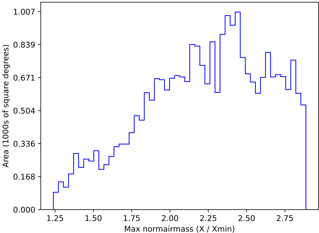
noroll_mjdp365_v3.4_10yrs All sky all bands: Max normairmass
