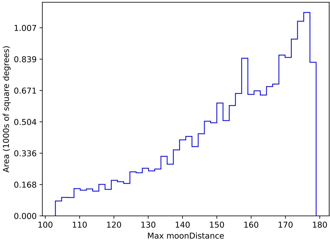
noroll_mjdp365_v3.4_10yrs WFD z band: Max moonDistance
