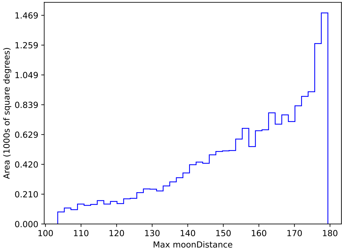
noroll_mjdp365_v3.4_10yrs WFD r band: Max moonDistance
