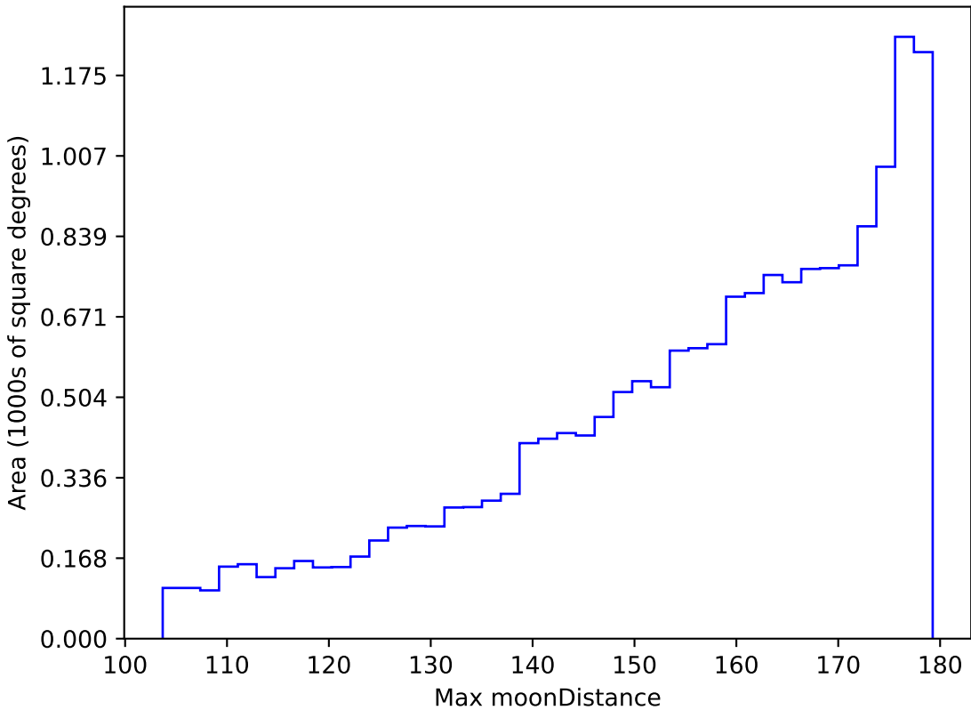
noroll_mjdp365_v3.4_10yrs WFD i band: Max moonDistance
