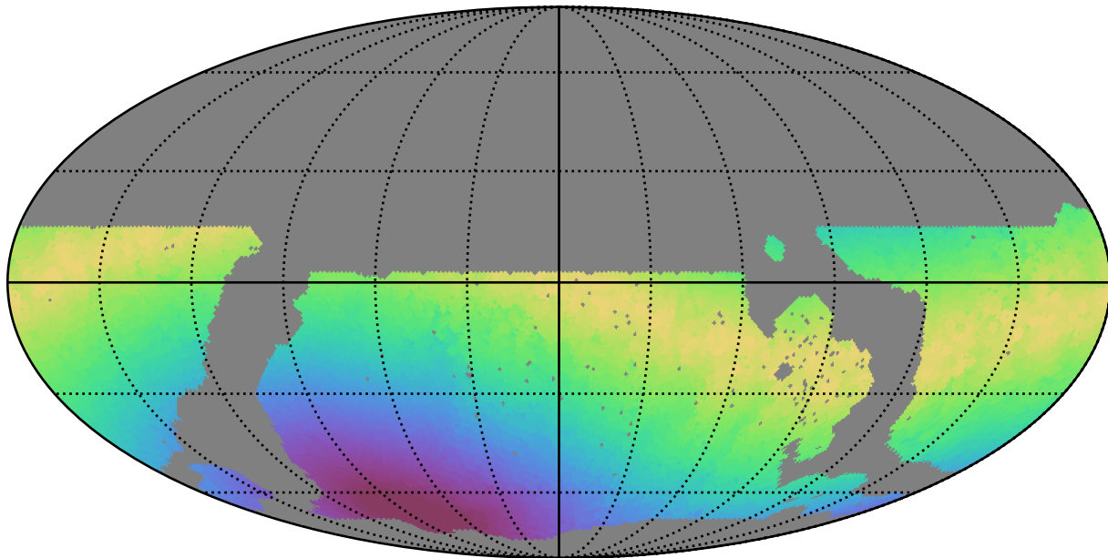
noroll_mjdp365_v3.4_10yrs WFD g band: Max moonDistance
