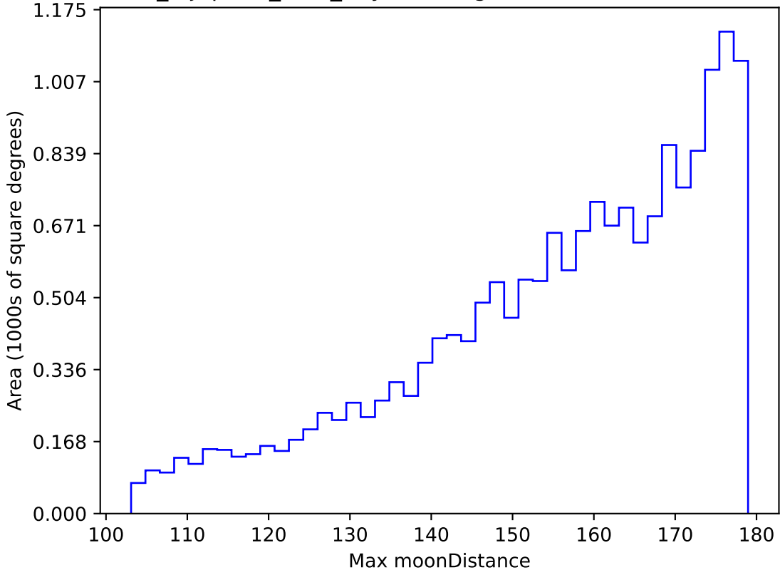
noroll_mjdp365_v3.4_10yrs WFD g band: Max moonDistance
