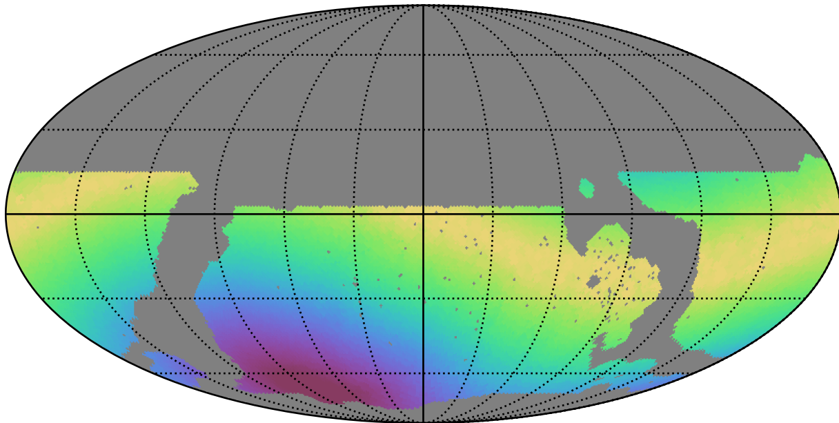
noroll_mjdp365_v3.4_10yrs WFD all bands: Max moonDistance
