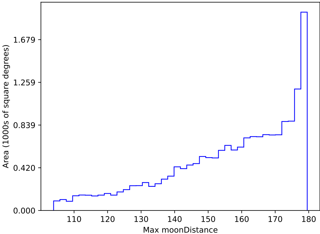
noroll_mjdp365_v3.4_10yrs WFD all bands: Max moonDistance
