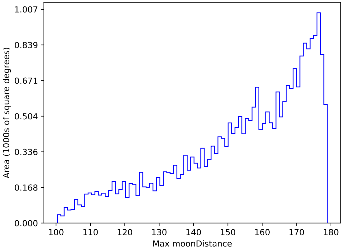
noroll_mjdp365_v3.4_10yrs All sky z band: Max moonDistance
