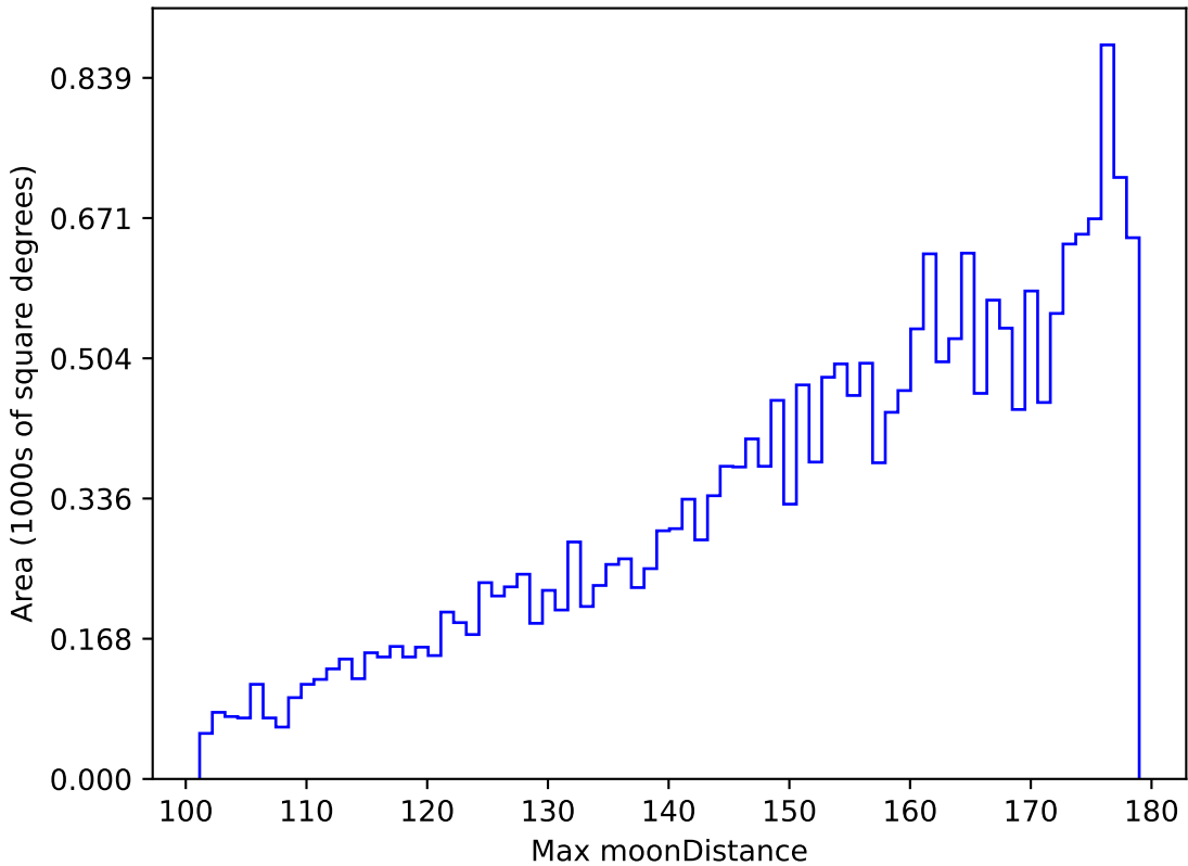
noroll_mjdp365_v3.4_10yrs All sky u band: Max moonDistance
