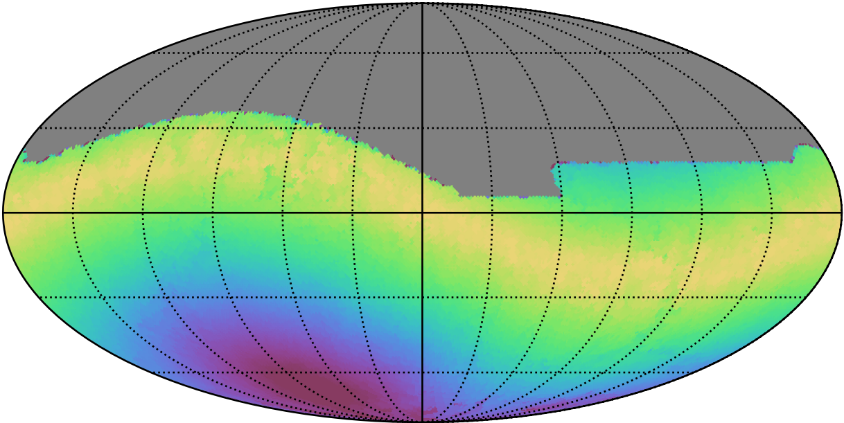
noroll_mjdp365_v3.4_10yrs All sky r band: Max moonDistance
