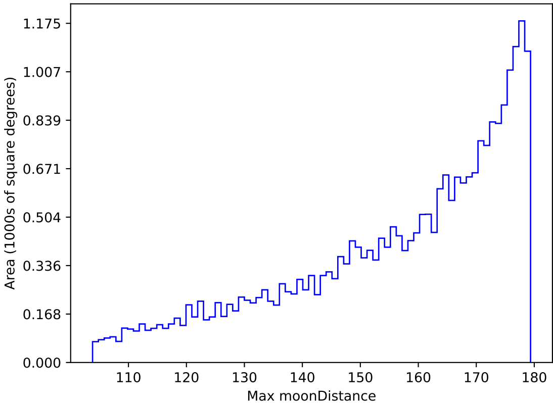
noroll_mjdp365_v3.4_10yrs All sky r band: Max moonDistance
