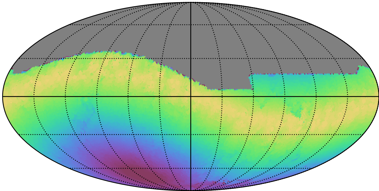
noroll_mjdp365_v3.4_10yrs All sky i band: Max moonDistance
