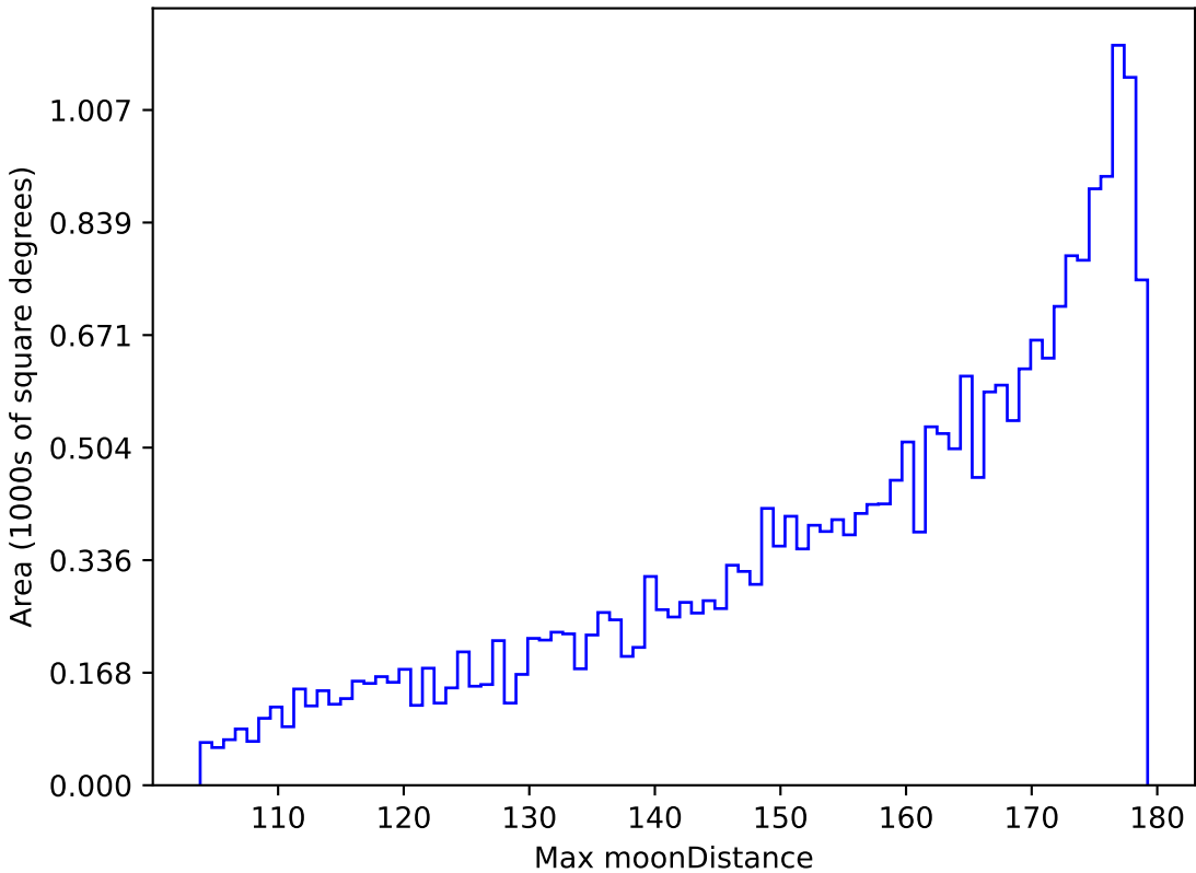
noroll_mjdp365_v3.4_10yrs All sky i band: Max moonDistance
