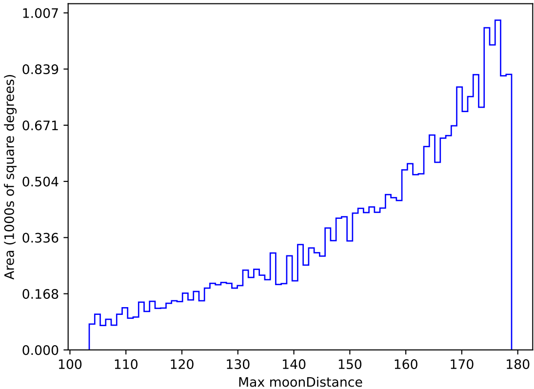
noroll_mjdp365_v3.4_10yrs All sky g band: Max moonDistance
