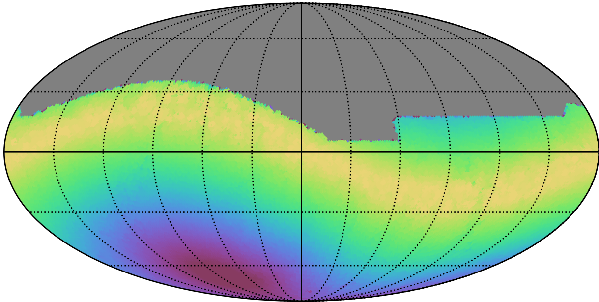
noroll_mjdp365_v3.4_10yrs All sky all bands: Max moonDistance
