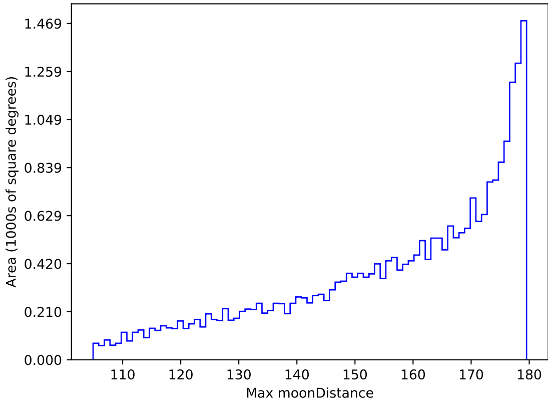
noroll_mjdp365_v3.4_10yrs All sky all bands: Max moonDistance
